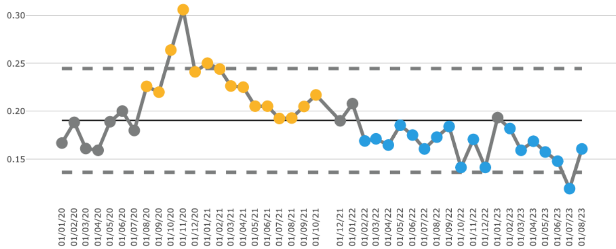
SPC Chart - CVC Target
